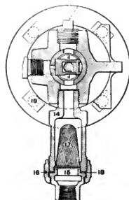
Fig. 2507. High-Speed Reducing Valve. Top View in Section.
